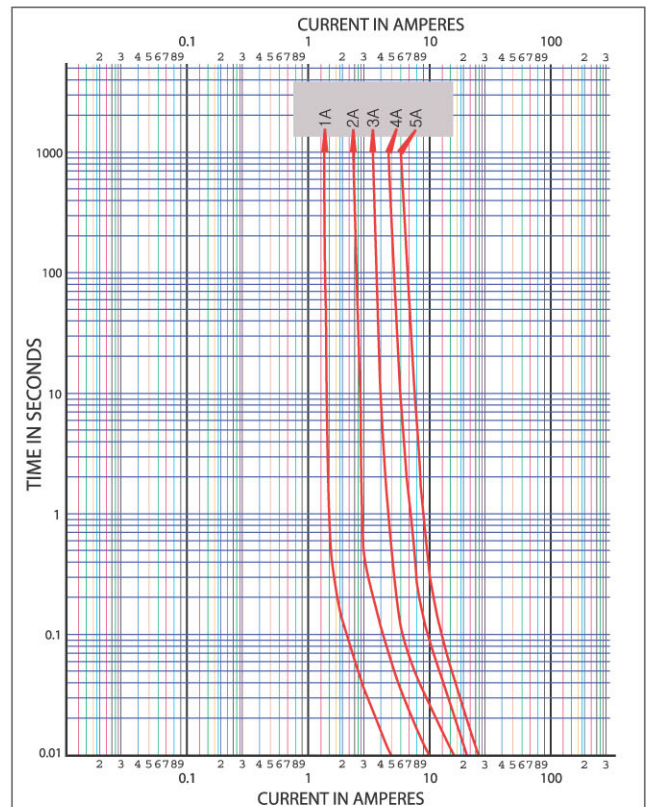
TIME-CURRENT CHARACTERISTICS
