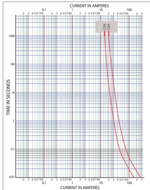
TIME-CURRENT CHARACTERISTICS
